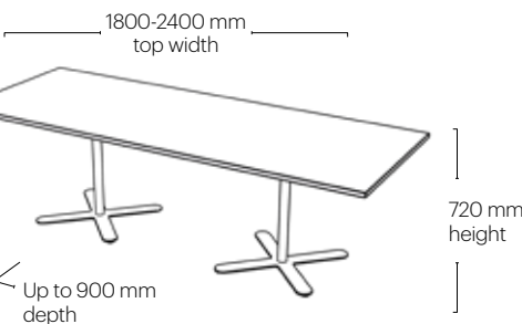
Bud Rectangular Table 720h BUD-720H-REC9-18-24
